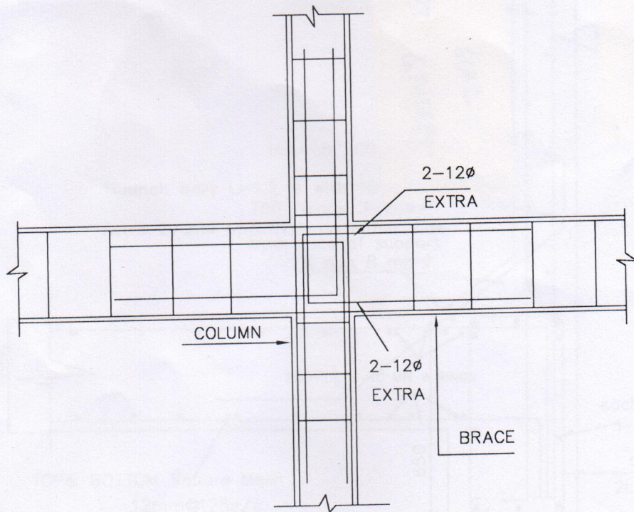
TYPICAL COLUMN BRACE JUNCTION
